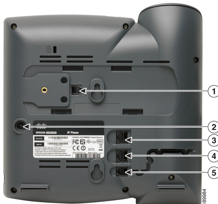
Figure 1 Cisco SPA 525G/525G2 IP Phone Connections
